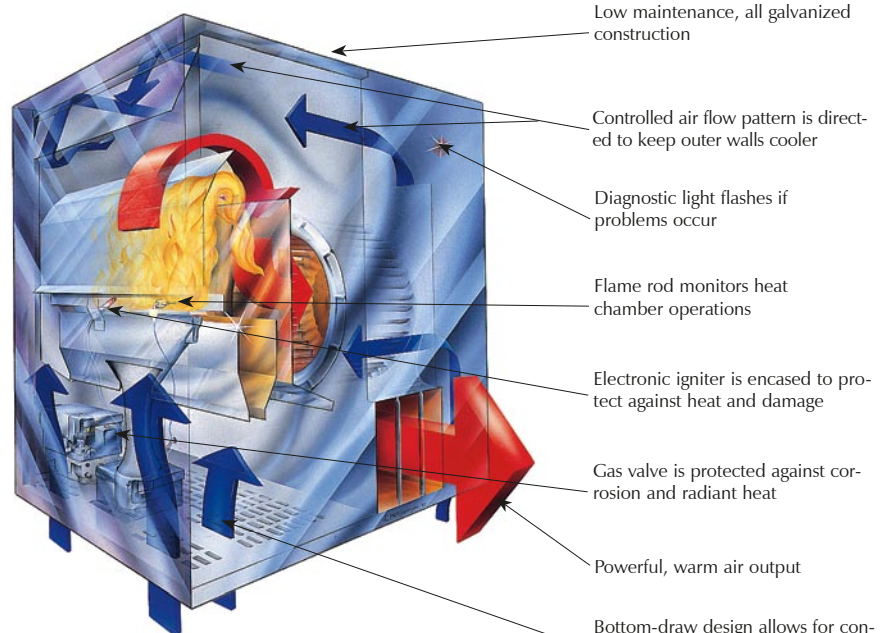
The "matchless" heater
